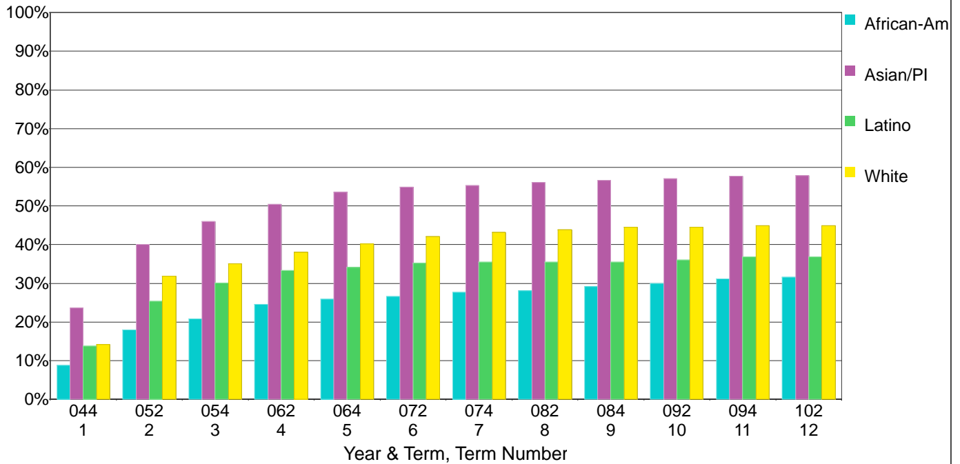
Cumulative Percentage Earning 12 or more College Level Units for the Fall 2004 First-Time College Cohort by Ethnicity and Term
